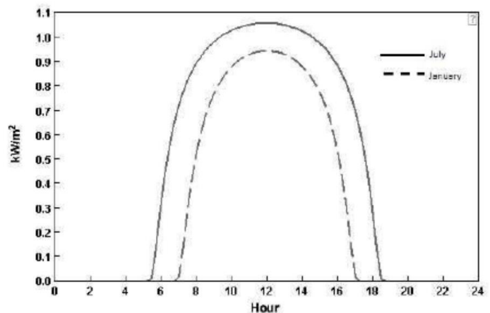
Fig-1: the lowest and the highest intensity of radiation in W/m 2
