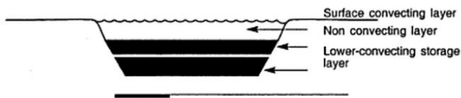
Fig-3: Salt-gradient solar pond The solar plant has normally three layers. In the first layer convection takes place due to wind evaporation. In the second layer salt gradient is used and make it non-convective this layer is 1m thick and in the final layer is convective layer which is act as thermal storage. A saturated pond is some time used for maintaining solubility of salt in water [19].
