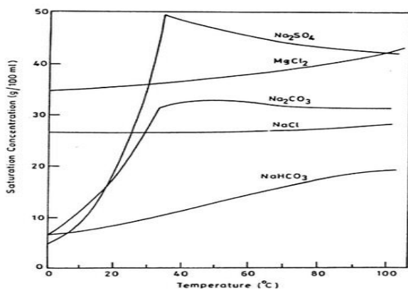
Fig-4: solubility of salts in water It was estimated that 100m-diameter solar pond which has 1m deep storage layer can be drive a Ranking cycle cooling unit to meet the air-conditioning needs of 50 homes [20]. This solar pond process can be useful in some cases where adequate solar energy is not available at all the time.
